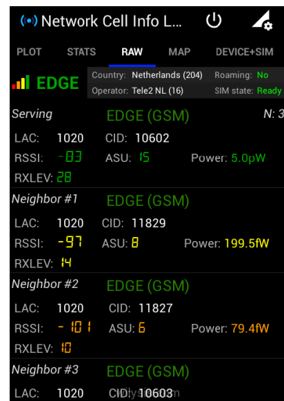
Figure 10: Phone connected to EDGE (2.75G) instead of the fake base station.
