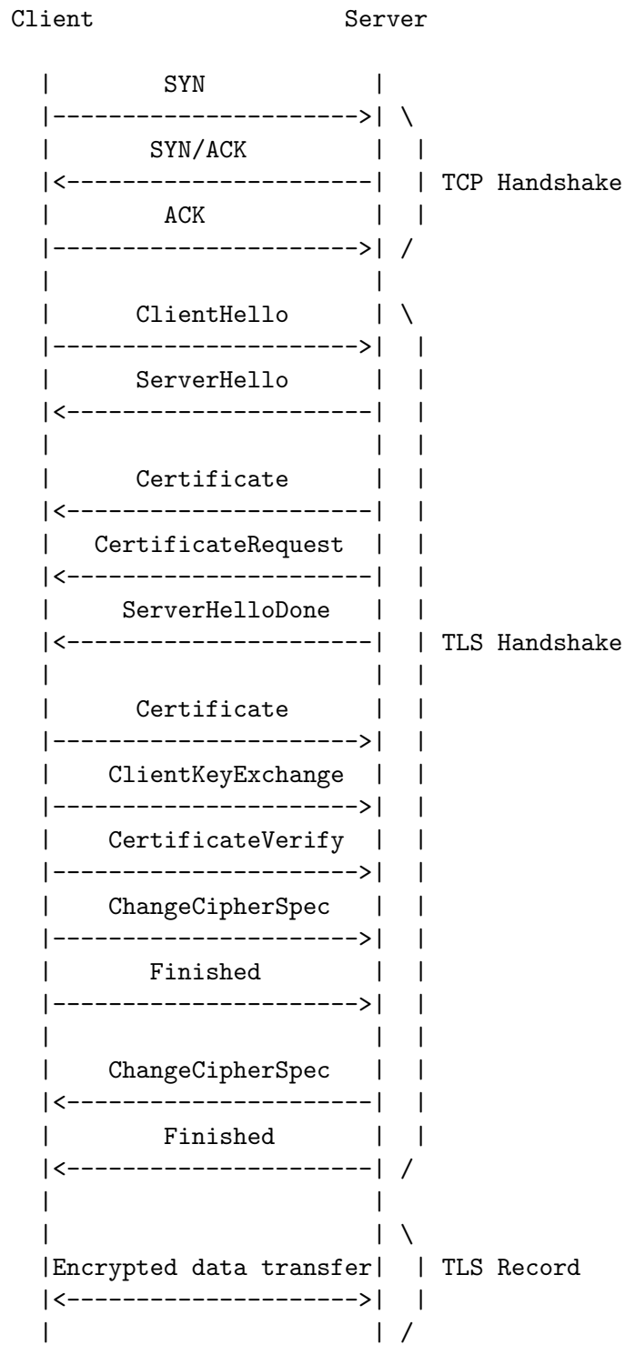
Figure 1: TLS flowchart
