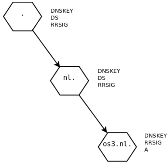
Figure 2: DNSSEC chain-of-trust
